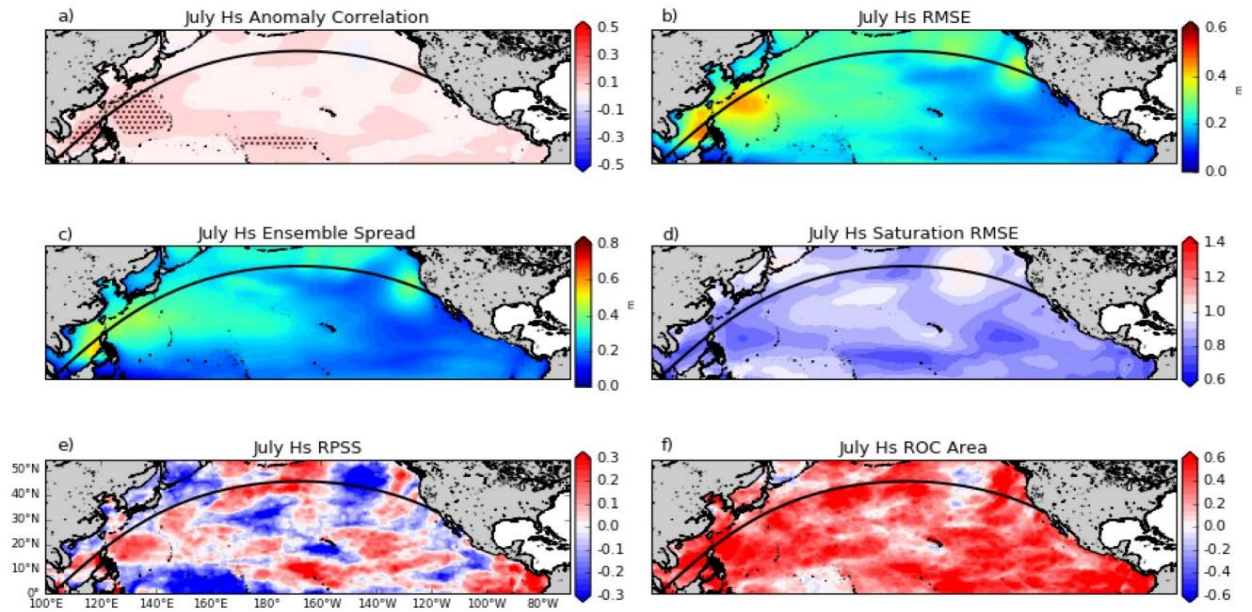
Figure 3: CCSM4-WW3 skill of simulating July significant wave height ( H_s ) compared to ERA-Interim using July initial condition. a) Anomaly correlation; b) Root Mean Square Error; c) Ensemble spread; d) Saturation Root Mean Square Error; e) Rank Probability Skill Score and f) Normalized Relative Operating Characteristic Area. The stippling on the anomaly correlation shows areas where the correlation coefficient is significantly different from zero at the 95-percentile level.
