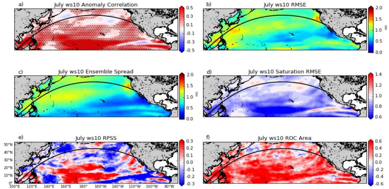
Figure 2: CCSM4 skill of simulating July 10m wind speed compared to ERA-Interim using July initial condition. a) Anomaly correlation; b) Root Mean Square Error; c) Ensemble spread; d) Saturation Root Mean Square Error; e) Rank Probability Skill Score and f) Normalized Relative Operating Characteristic Area. The stippling on the anomaly correlation shows areas where the correlation coefficient is significantly different from zero at the 95-percentile level.
